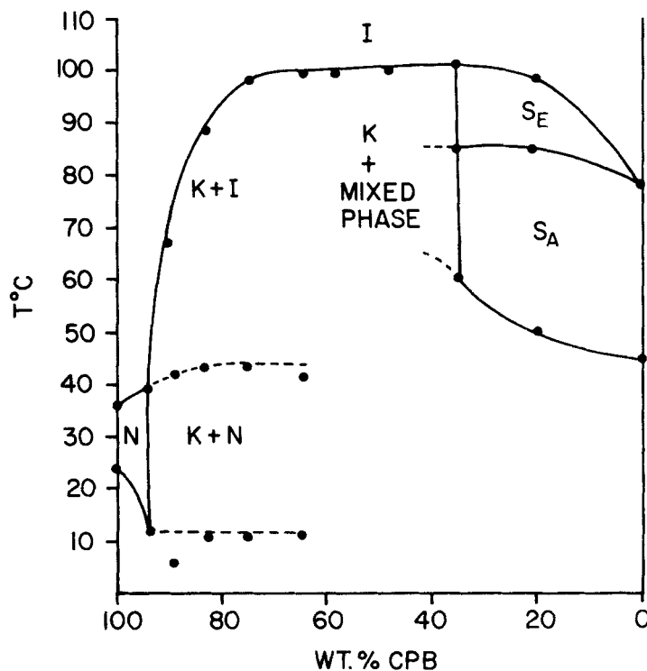
Figure 1. Phase Diagram for the Binary System CPB and V
